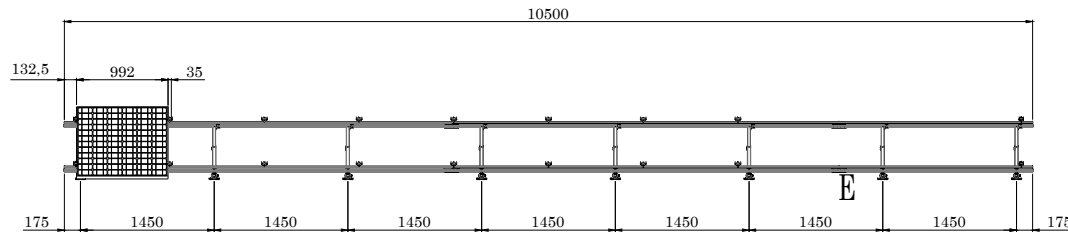
VISTA FRONTAL
