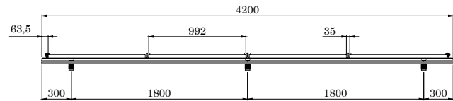
VISTA FRONTAL
