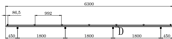
VISTA FRONTAL
