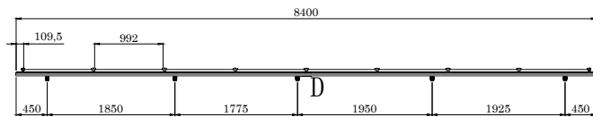
VISTA FRONTAL
